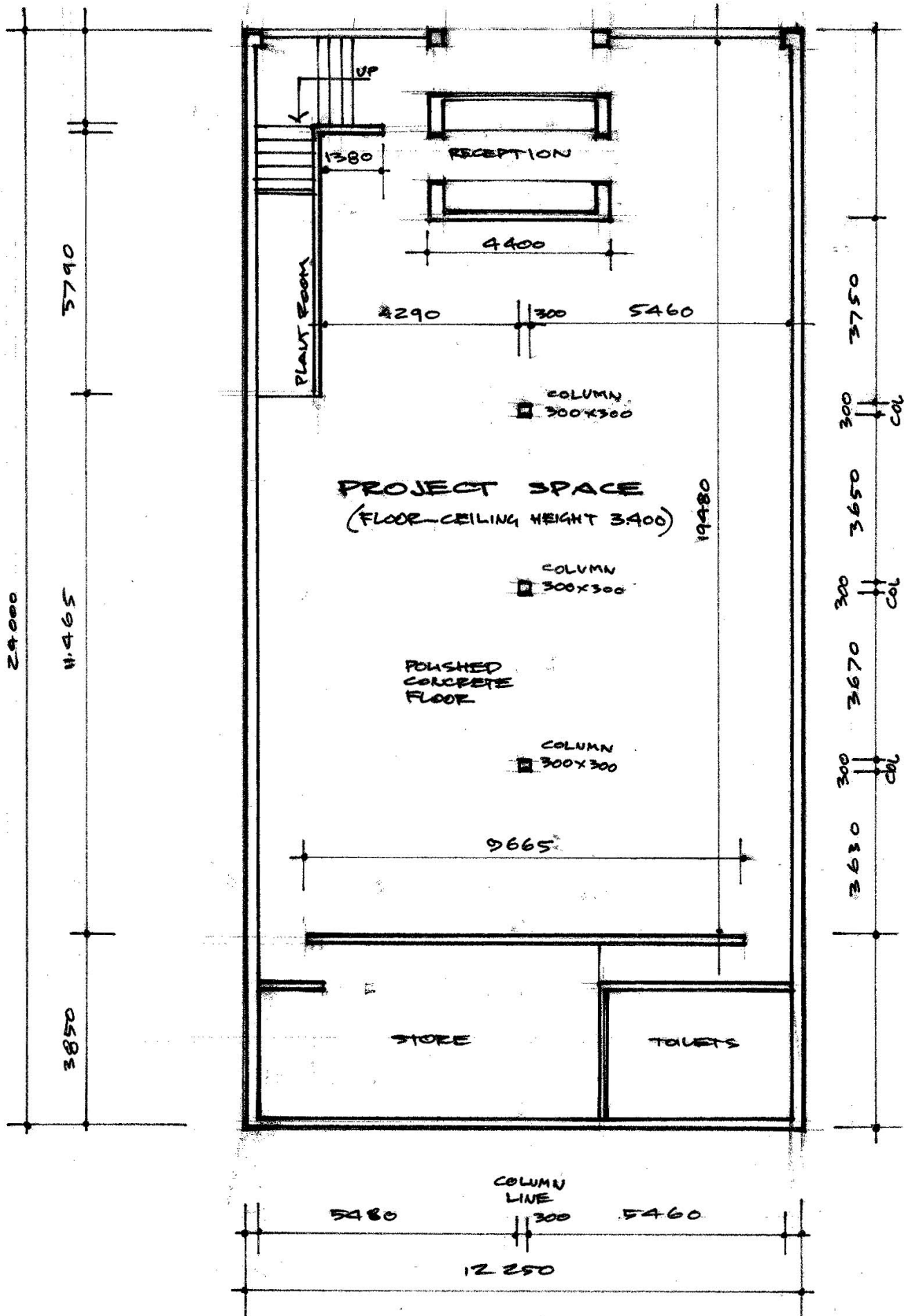
GROUND FLOOR PLAN-TWO ROOMS SCALE 1:100
